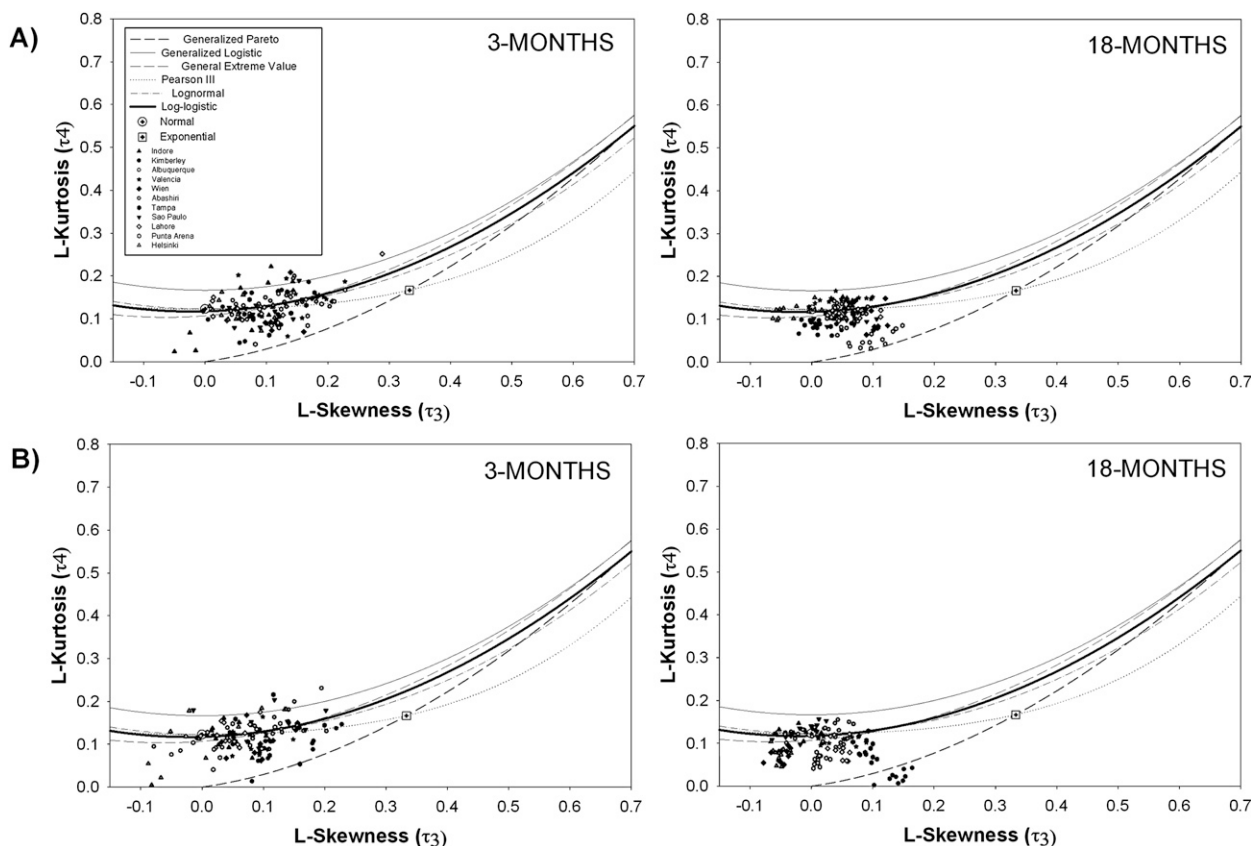
FIG. 13. L-moment ratio diagrams for the D series calculated at the time scales of 3 and 18 months. Progressive temperature increase of (a) 2° and (b) 4°C. The theoretical L-moment ratios for different distributions are shown, as are the empirical values obtained from the monthly series at each observatory.
